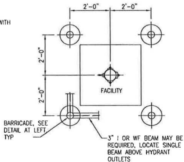
BOLLARD/BARRICADE PLAN
