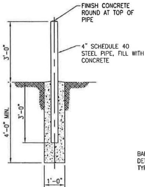
BOLLARD/BARRICADE DETAIL
