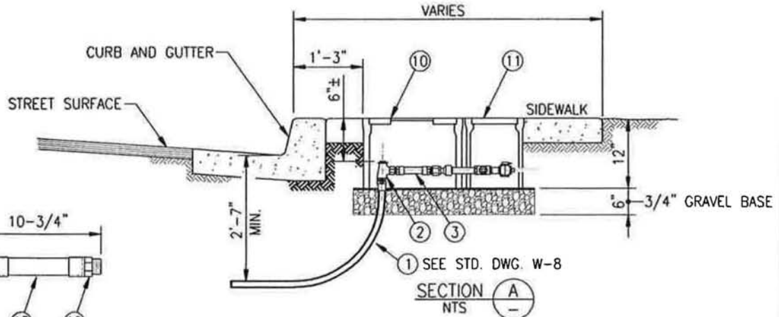
METER IDLER (JUMPER) DETAIL (1) NTS
