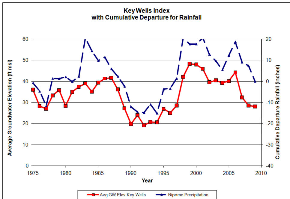
Figure 7-1. Key Wells Index with cumulative departure for rainfall (using average rainfall from the combination of gauges at Nipomo CDF #151.1 and Mehlschau #38). The two graphs are plotted
