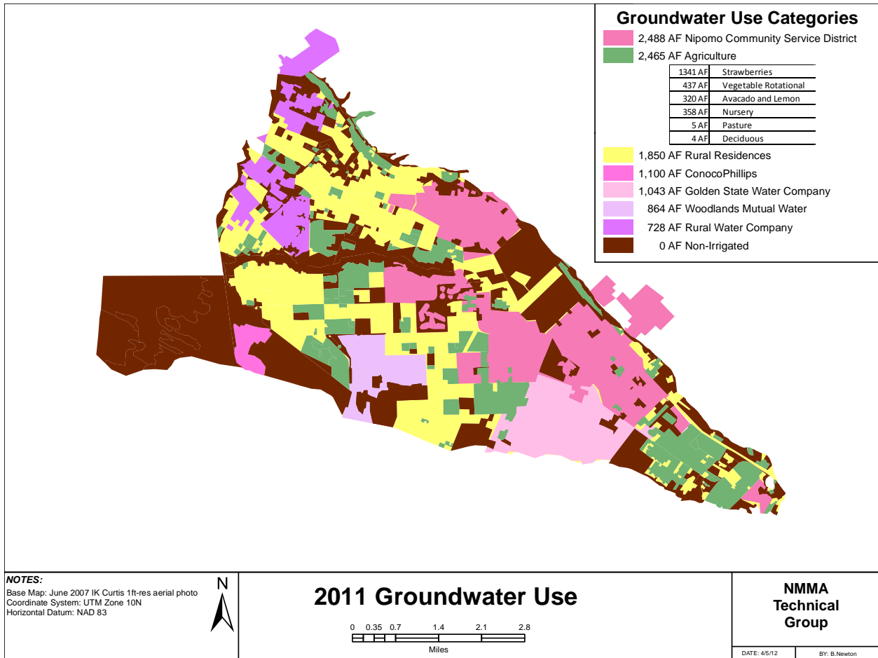
Figure 3-7. 2011 Groundwater Use
