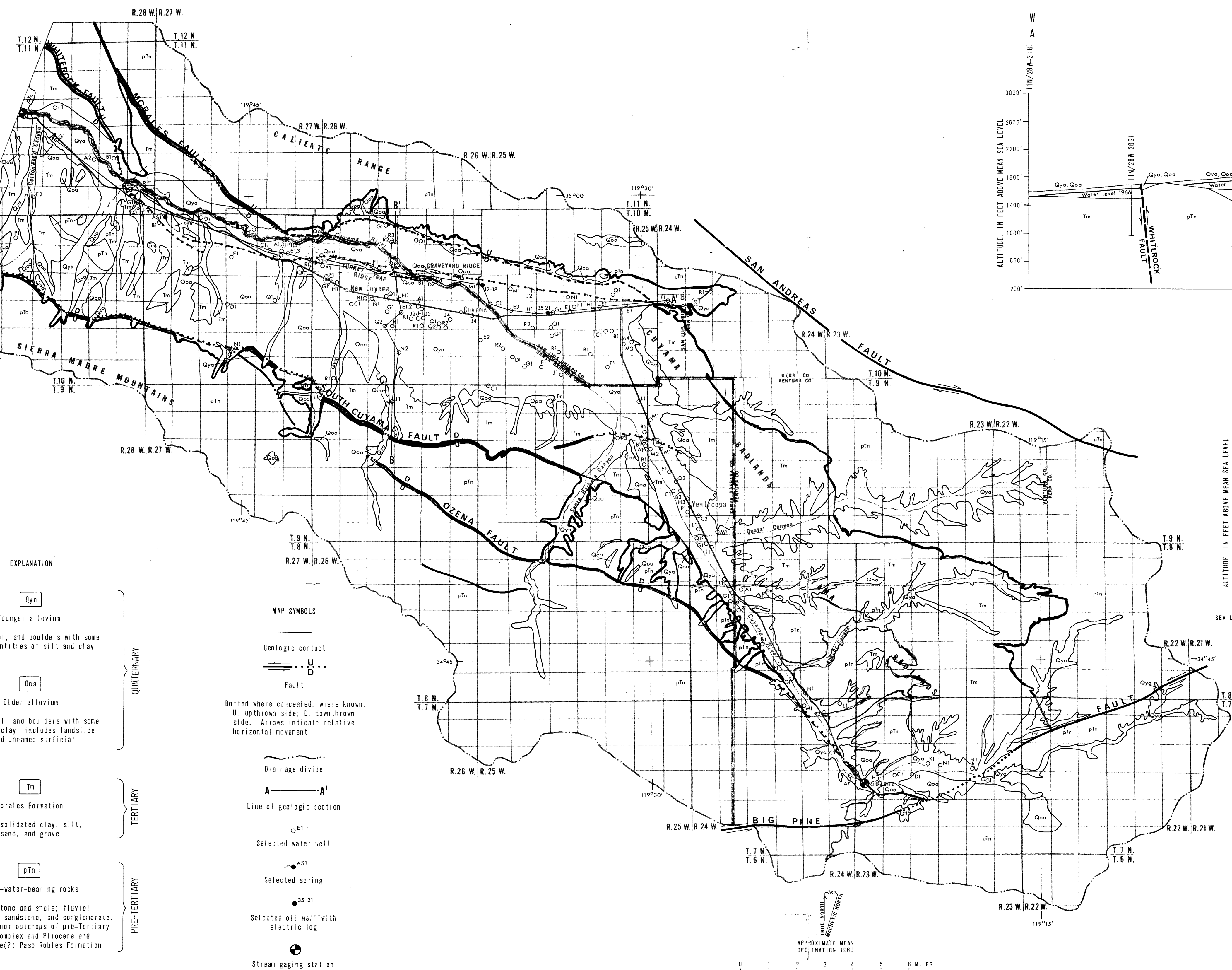
MAP OF CUYAMA VALLEY, CALIFORNIA, SHOWING GENERAL GEOLOGY, SELECTED WELLS, AND GEOLOGIC SECTIONS
