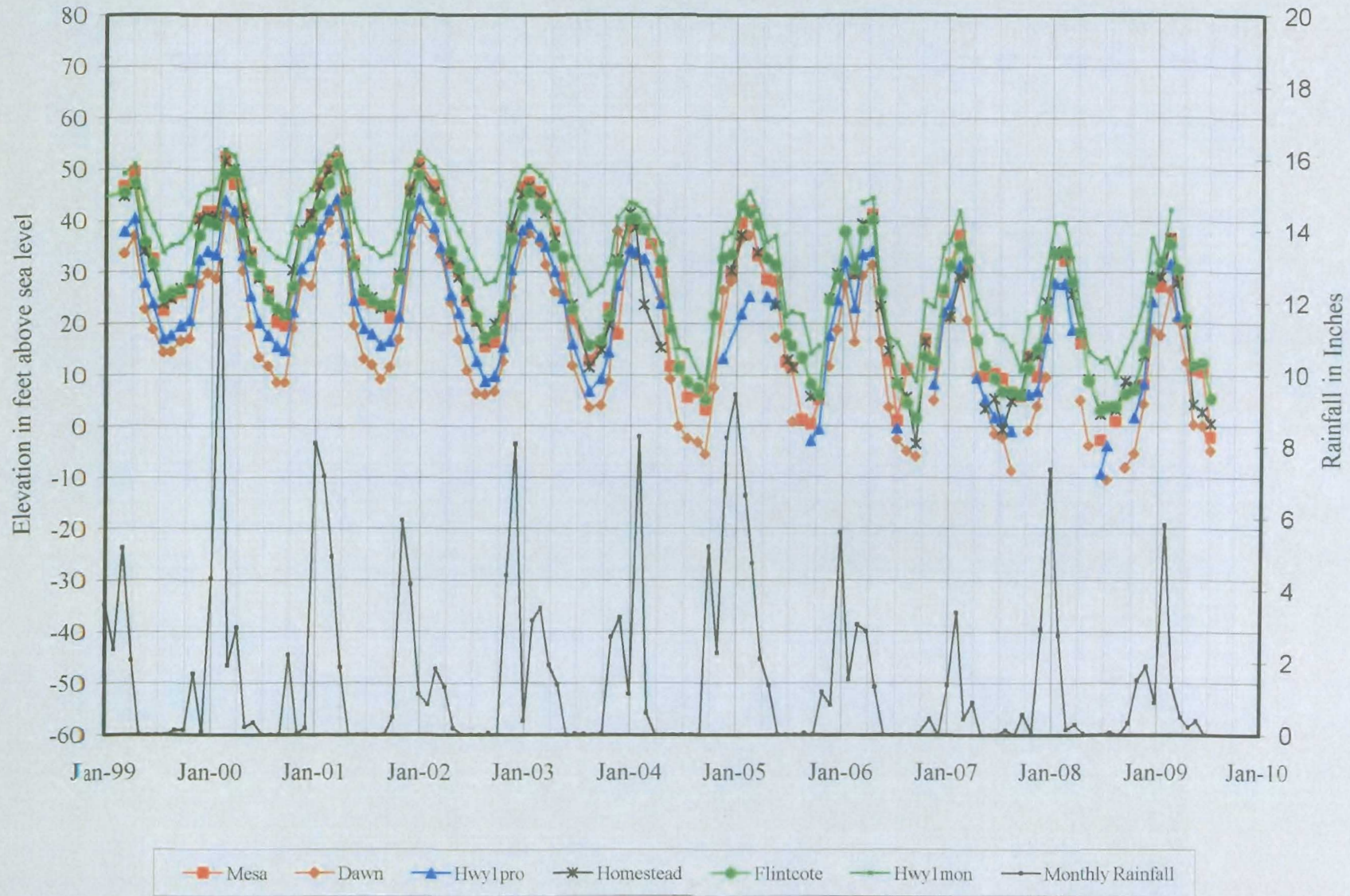
Figure 3 Water Levels: March 1999 to July 2009 The Woodlands Onsite Wells
