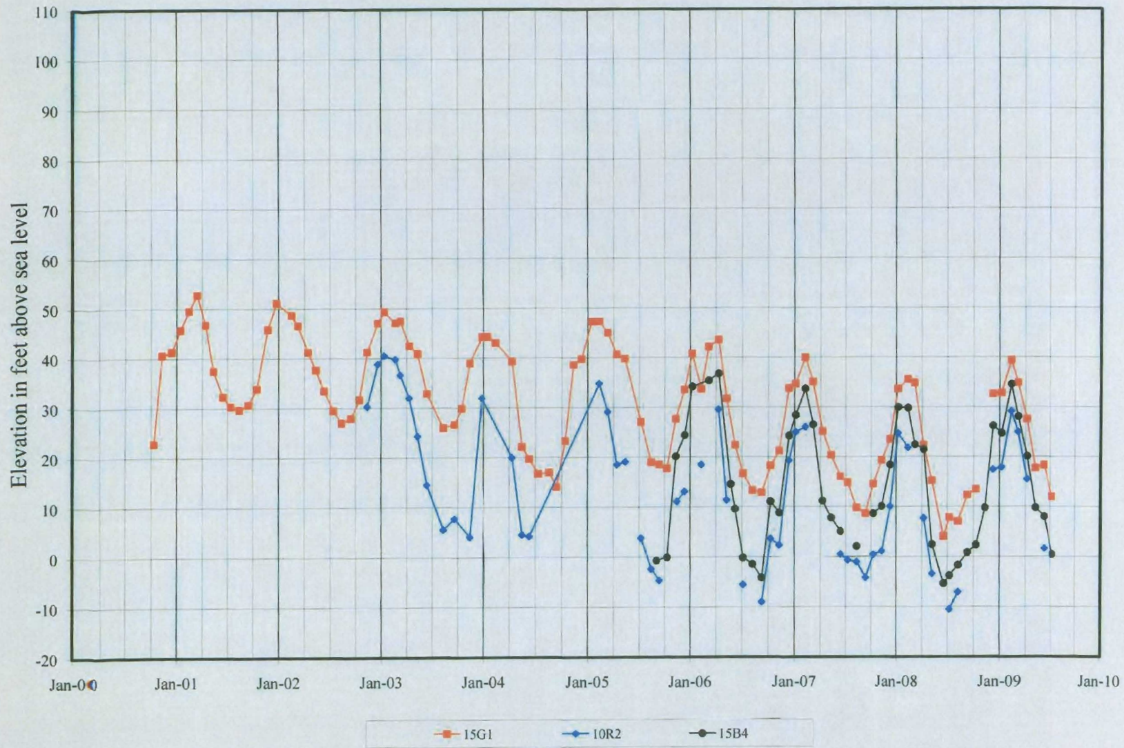
Figure 6 Water Levels Through July 2009 The Woodlands Offsite - Northeast Wells
