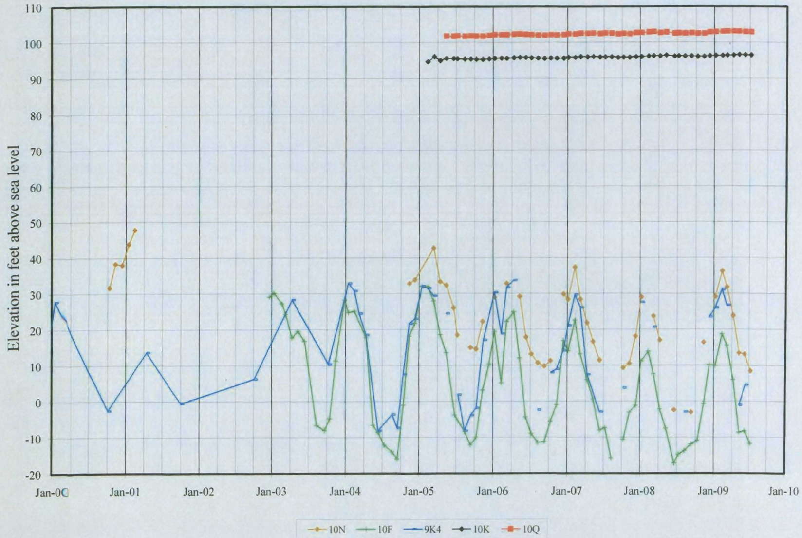
Figure 5 Water Levels Through July 2009 The Woodlands Offsite - Northern Wells
