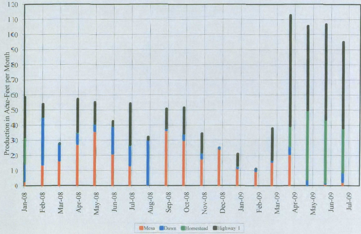
Figure 2 Well Production: January 2007 through July 2009 The Woodlands Onsite Wells
