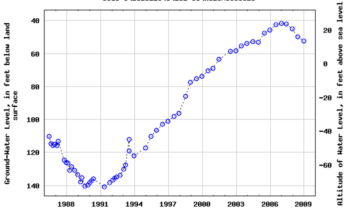
Figure 21: Hydrograph of State Well 4N/28W-9J2
