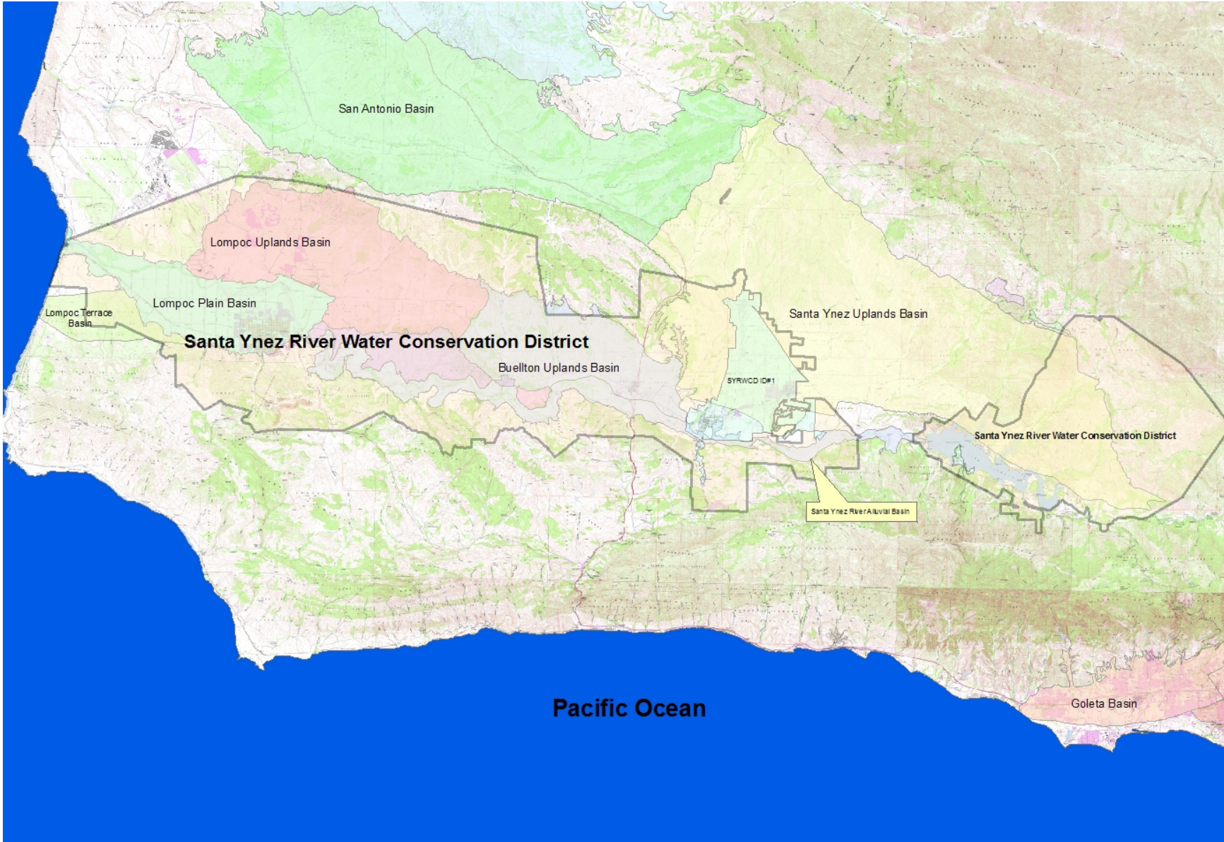
Figure 22: Santa Ynez River Water Conservation District Boundaries
