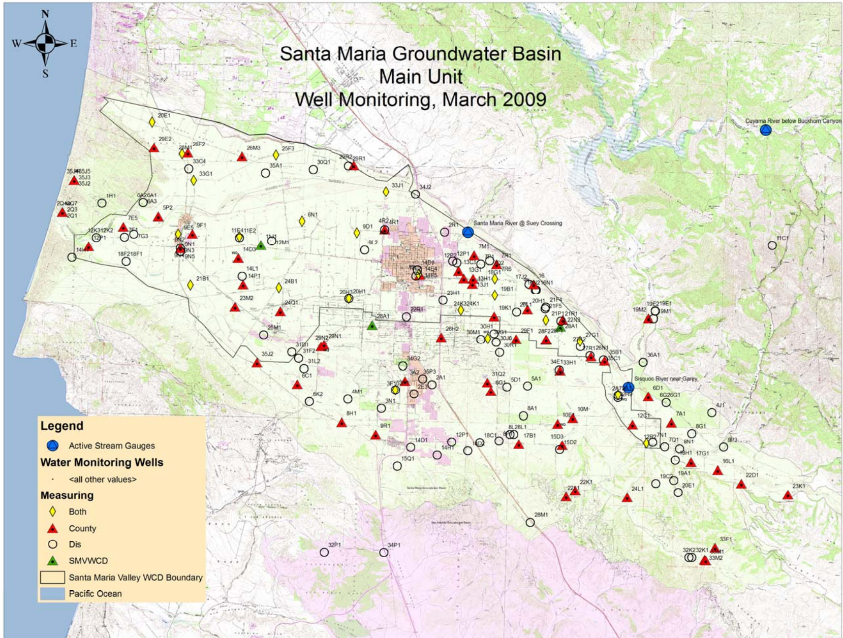
Figure 39: Distribution of Groundwater Monitoring Sites in the Santa Maria Valley
