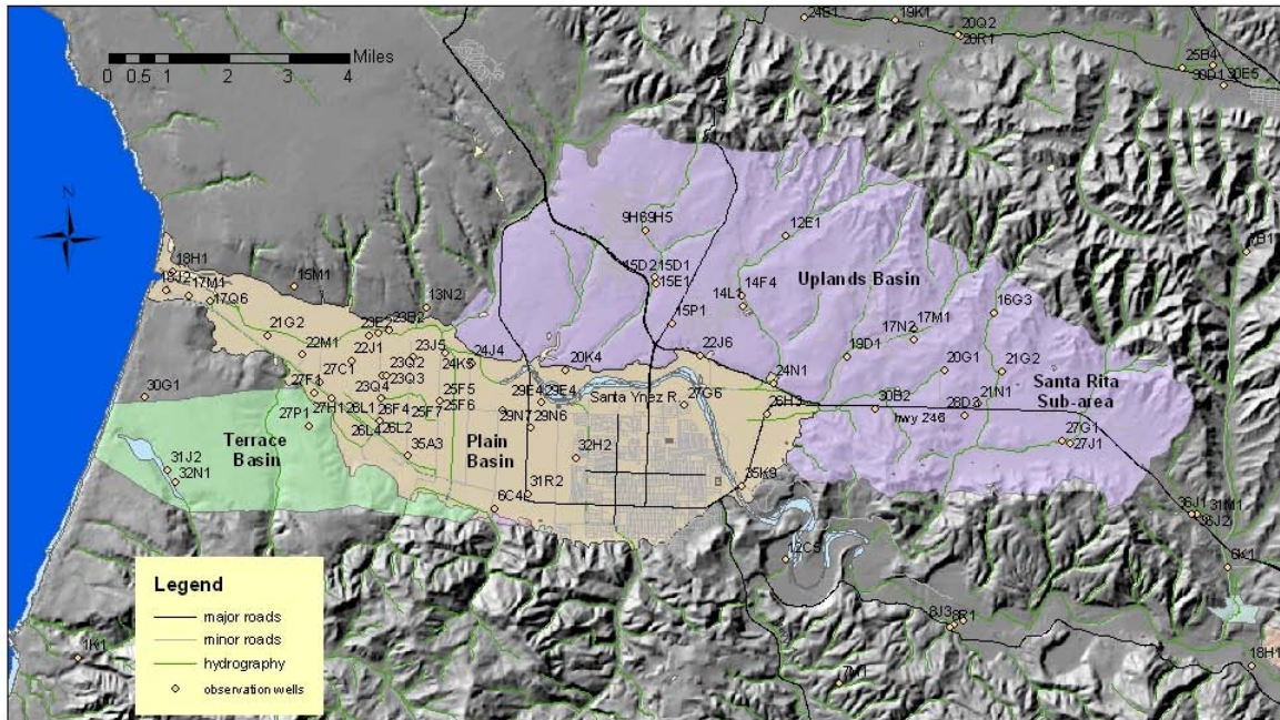
Figure 29: Lompoc Area Groundwater Basins
