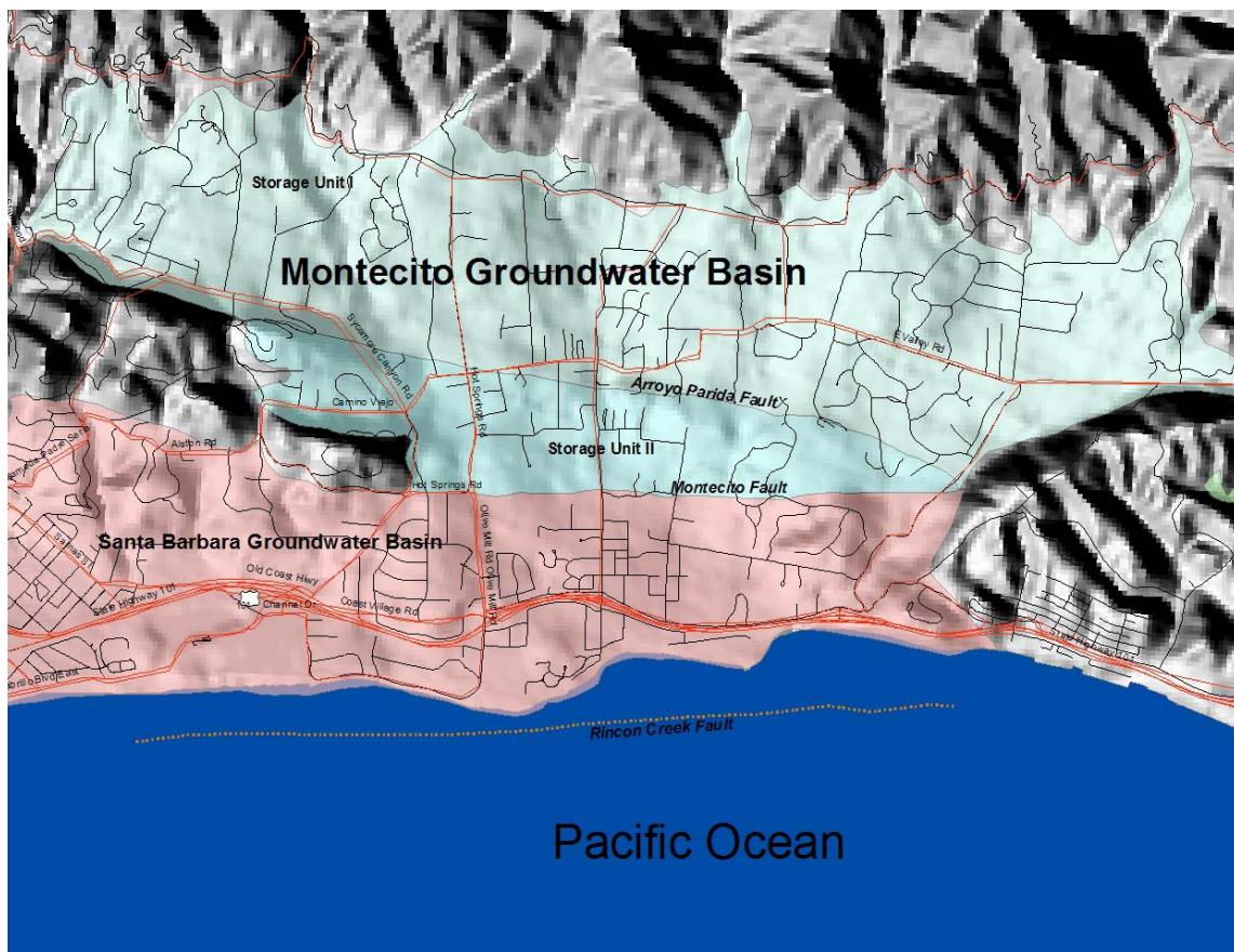
Figure 14: Montecito Groundwater Basin
