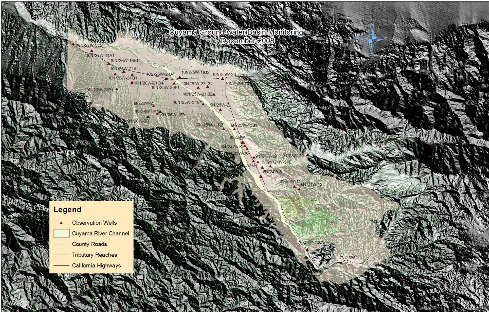
Figure 52: Cuyama Groundwater Basin
