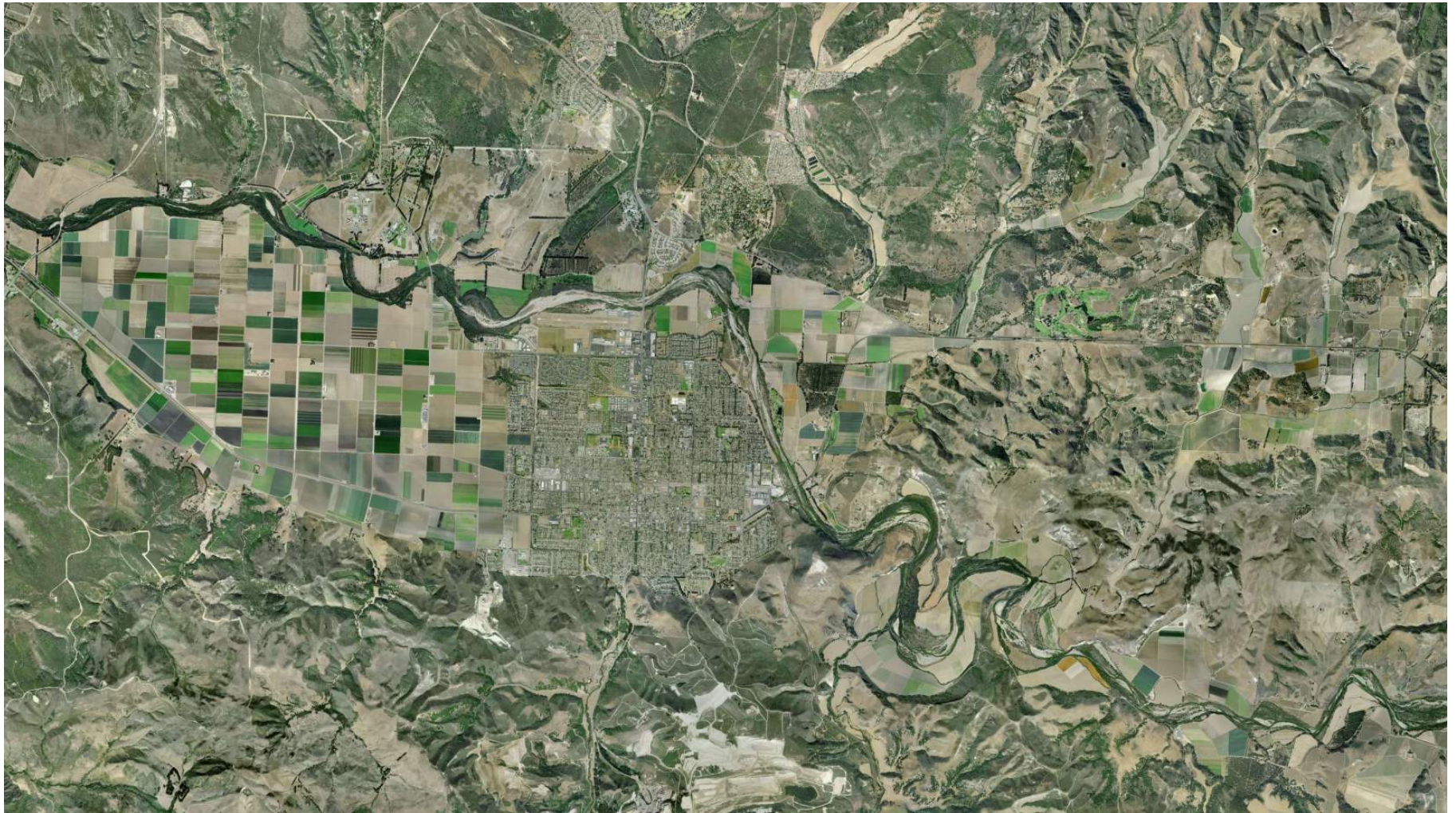
Figure 30: Aerial image of the Lompoc, Lompoc Uplands and Santa Rita Area taken in August of 2004. The Lompoc Plain Basin is adjacent and west of the urbanized area which is the City of Lompoc. The Lompoc Uplands which provide water to the communities of Vandenberg Village and Mission Hills lies to the north of the City and Lompoc Plain. The Santa Rita area is the easternmost section of the Basin and is hydrologically connected to the other Sub-basins by a geologic syncline the axis of which runs east-west.
