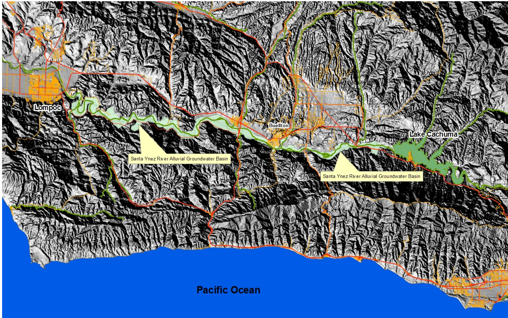
Figure 27: Santa Ynez River Alluvial Groundwater Basin
