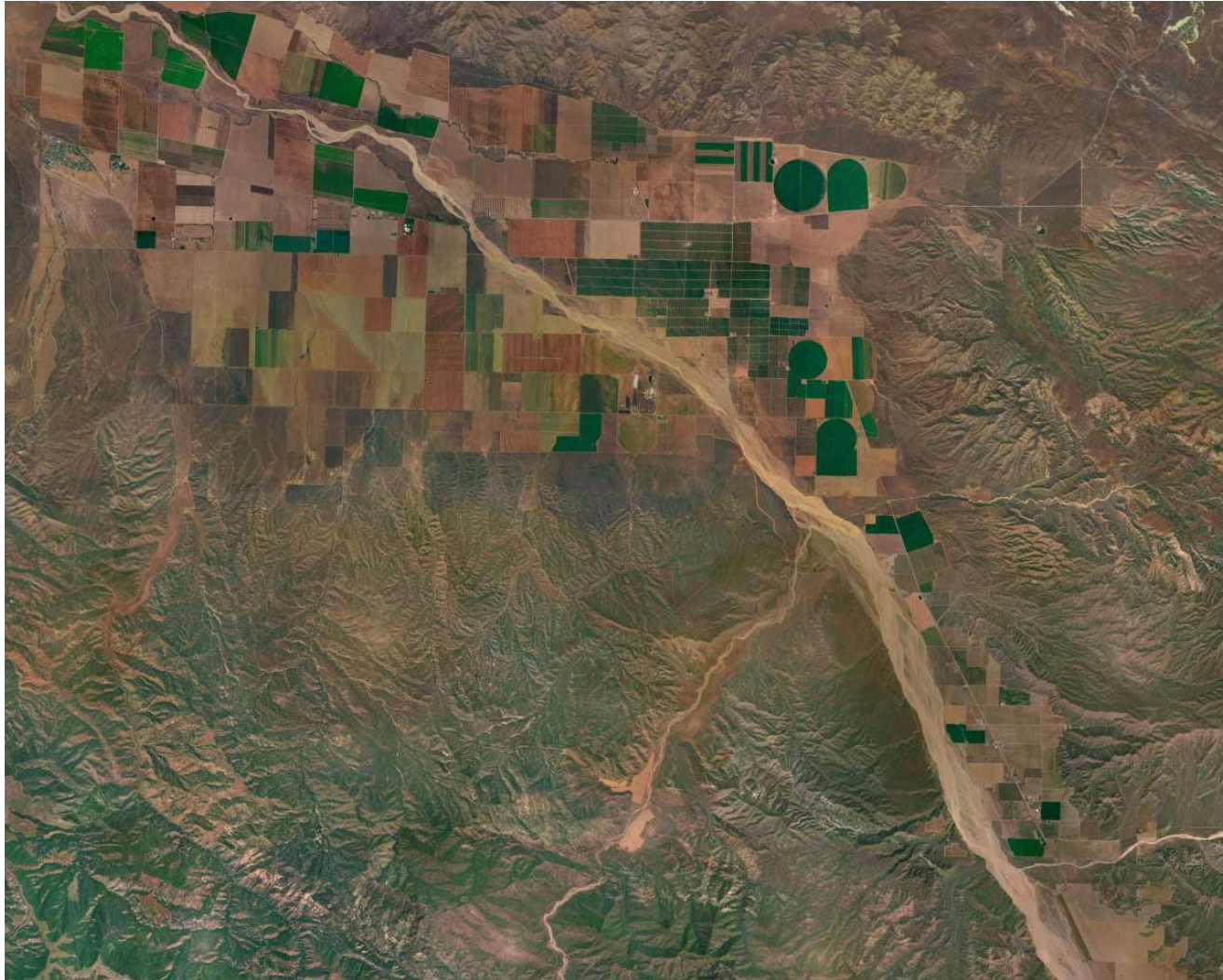
Figure 51: Aerial Photograph of the Cuyama River Valley
