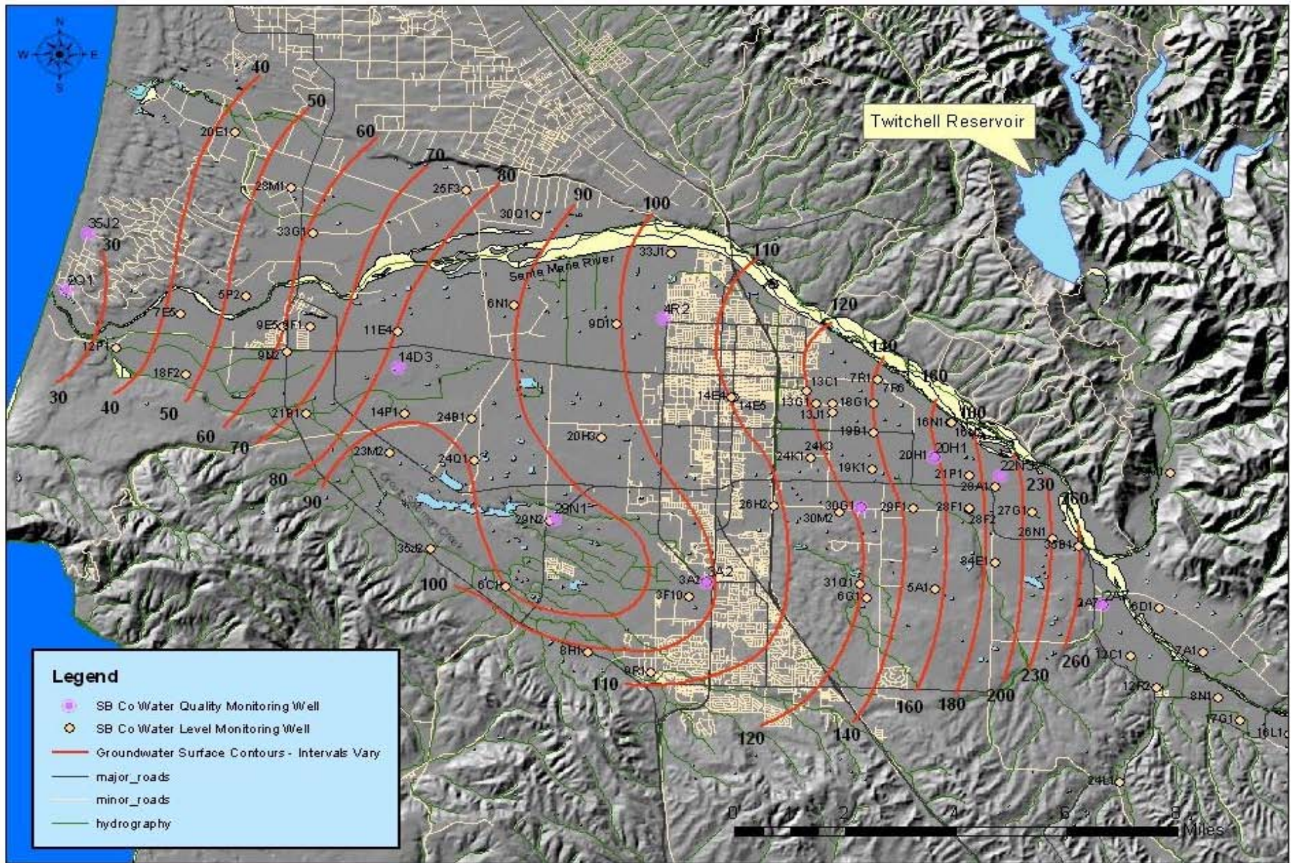
Figure 42: Spring 2004 Groundwater Level Contours for the Santa Maria Groundwater Basin Main Unit
