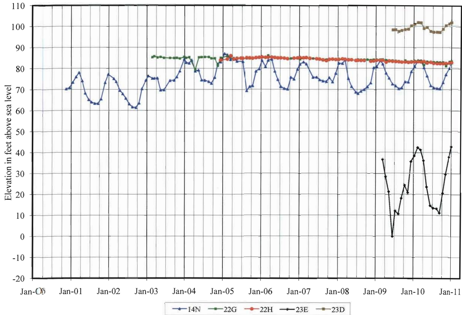
Figure 4 Water Levels Through January 2011 The Woodlands Offsite - Southeast Wells
