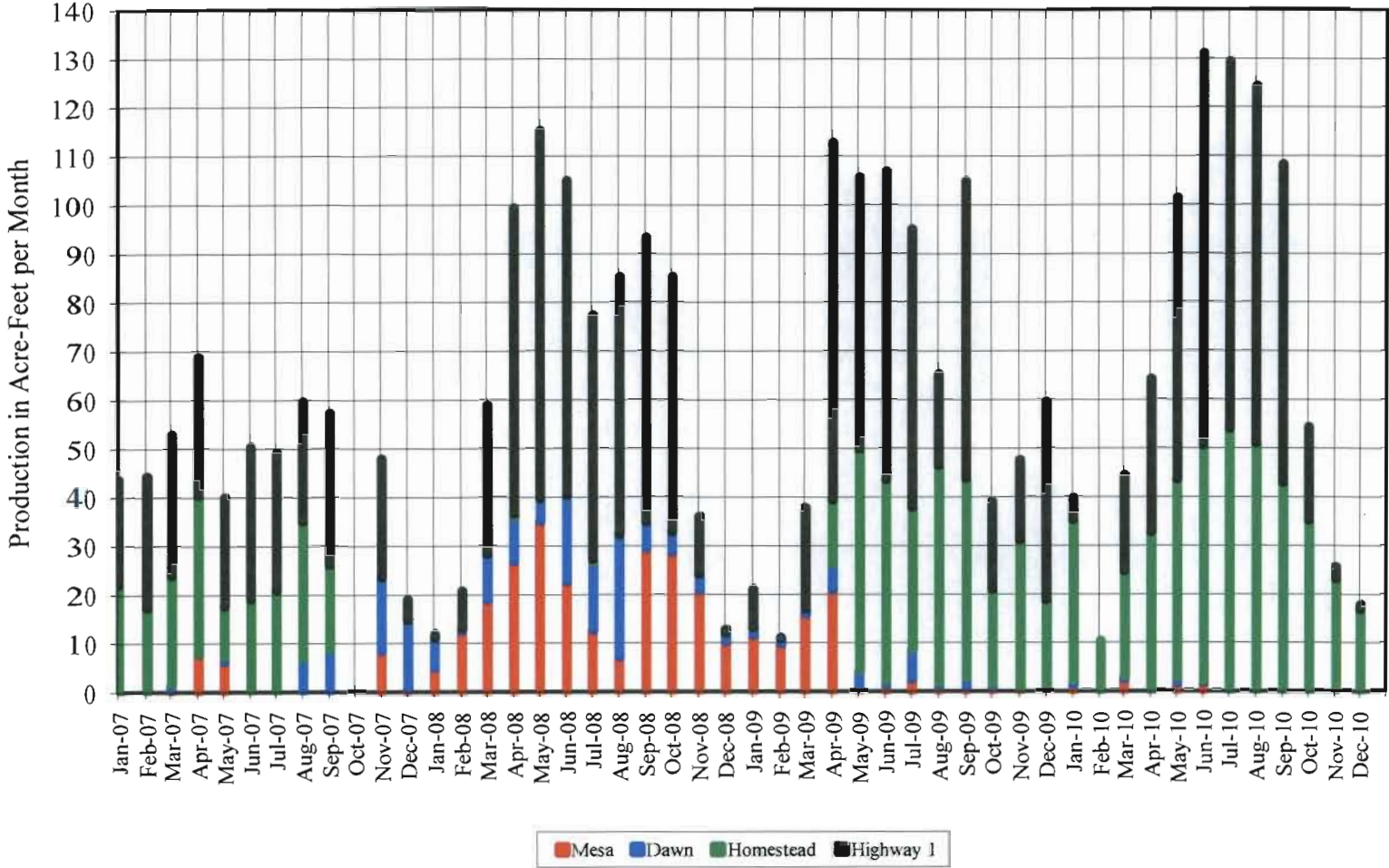
Figure 2 Well Production: January 2007 through December 2010 The Woodlands Onsite Wells
