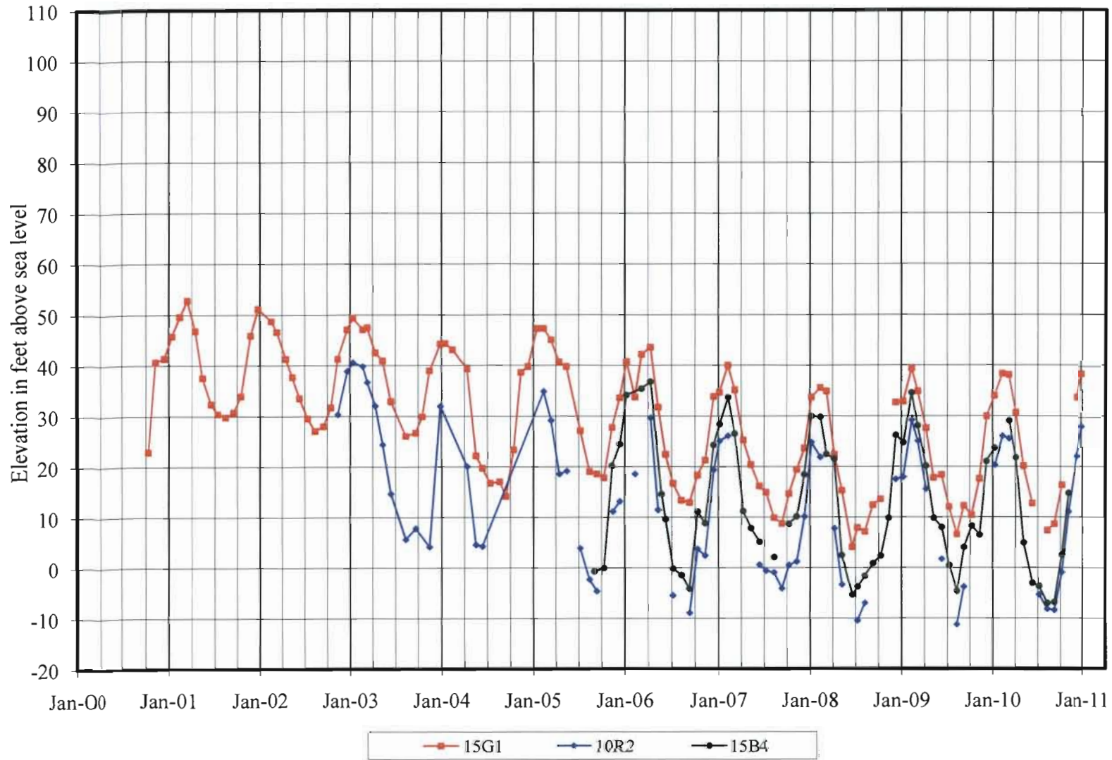
Figure 6 Water Levels Through January 2011 The Woodlands Offsite - Northeast Wells
