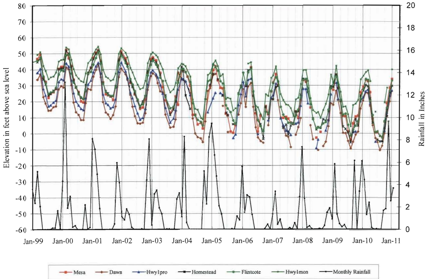
Figure 3 Water Levels: March 1999 to January 2011 The Woodlands Onsite Wells
