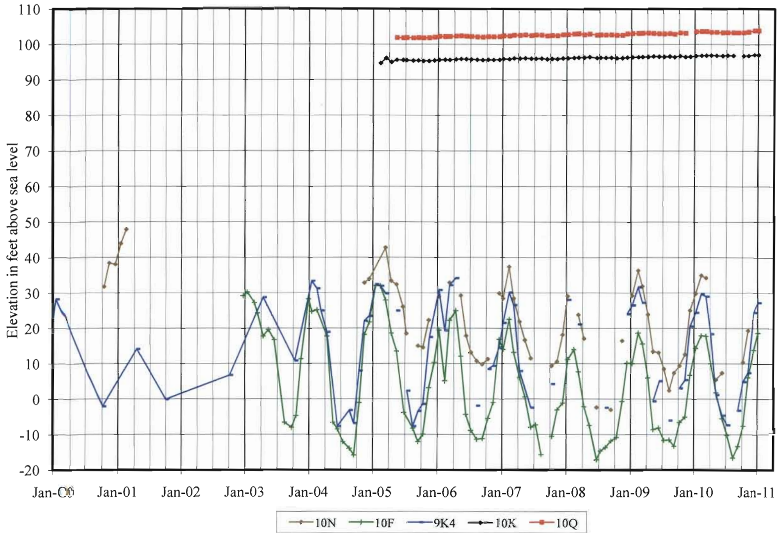
Figure 5 Water Levels Through January 2011 The Woodlands Offsite - Northern Wells
